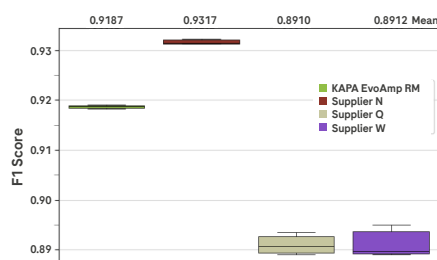
Figure 2. High precision and recall rates for reliable variant calling with KAPA EvoAmp ReadyMix powered by HiFi. A higher F1 score in variant calling indicates a better balance between precision and recall, reflecting the overall effectiveness of the variant-calling method. This allows researchers to focus on biologically meaningful findings rather than errors. Whole genome sequencing DNA libraries (10 ng Human genomic DNA, NA12878) were prepared using the KAPA EvoPrep Boost Kit and amplified with either KAPA EvoAmp ReadyMix or Supplier N, Supplier Q and Supplier W PCR mixes. (A) KAPA EvoAmp ReadyMix exhibits high SNP detection accuracy with low variability. (B) KAPA EvoAmp ReadyMix exhibits high consistency for Insertions/Deletions (InDels) detection accuracy.
